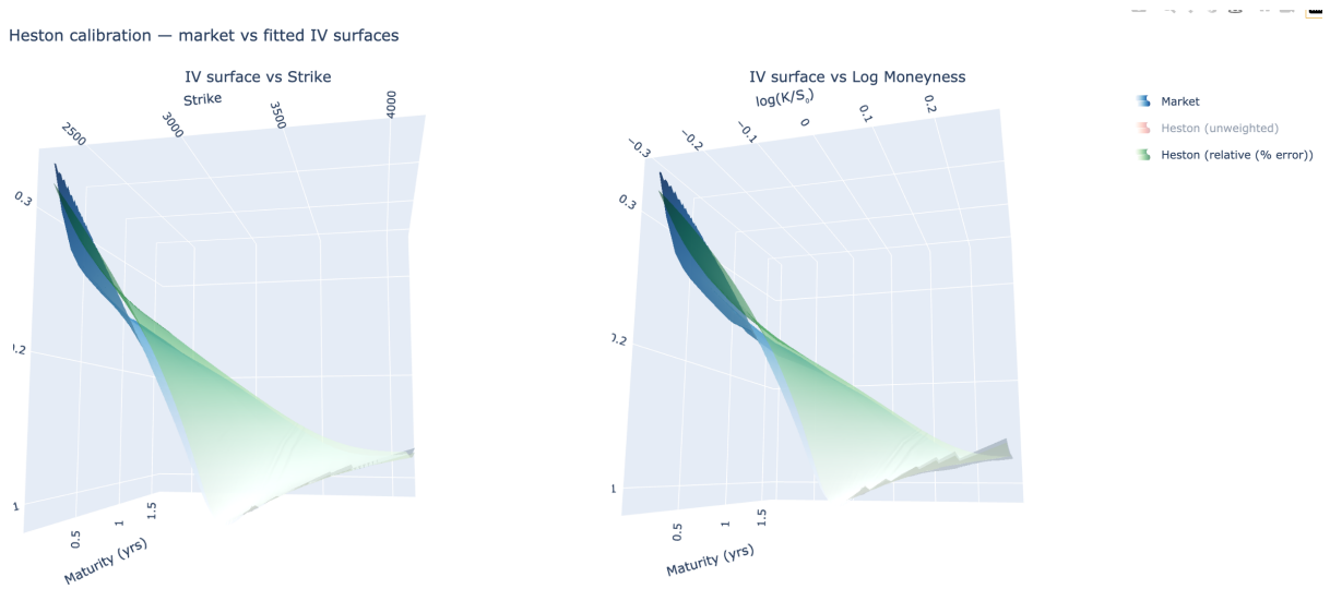
Figure A.7: Alternative viewing angle of the Heston fitted IV surface (relative error weighting) vs. market implied volatility surface, S&P 500 options (13 November 2019, S_0 = 3094 ).
